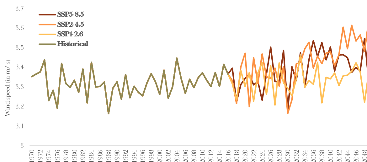
Figure 4: Historical and projected windspeed trends for Ratnagiri (1970–2050)
